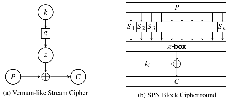
Figure 2: Encryption diagrams for Vernam-like stream ciphers and SPN block ciphers.
