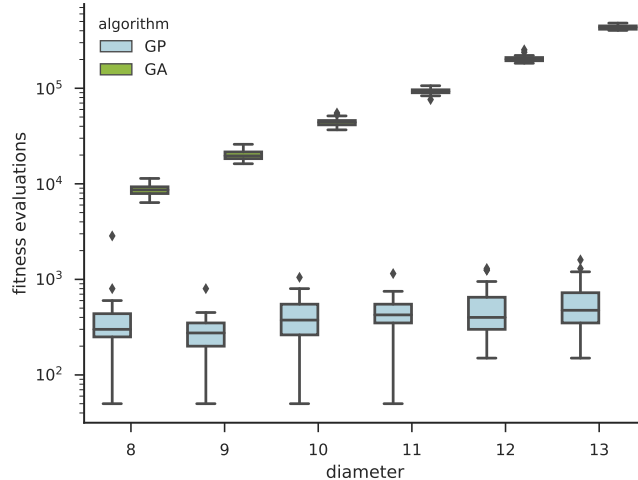
Figure 3: Comparison of fitness evaluations performed by GA and GP.
