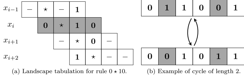
Figure 2: A locally invertible CA defined by the single landscape 0 \star 10 .
